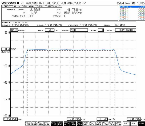
Optical Spectrum @50mW Output Power
