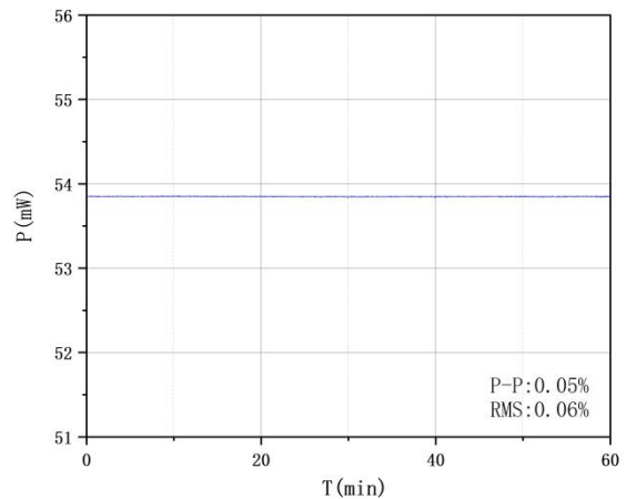
Power Stability @50mW Output Power
