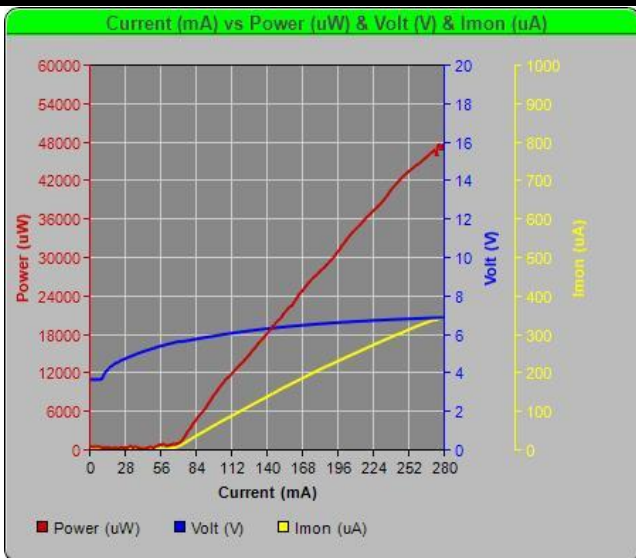
PIV Curve
