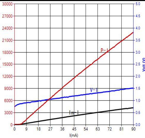
PIV Curve
