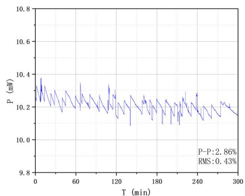
Power Stability @10mW Output Power
