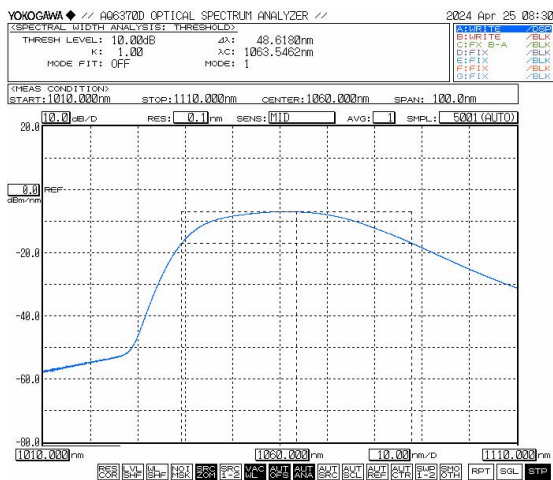
Optical Spectrum @10mW Output Power
